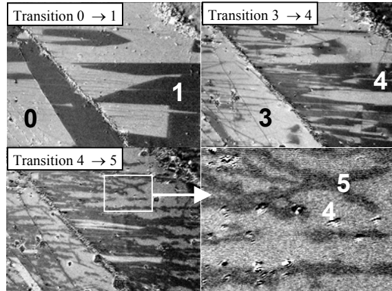
Fig.3 Magnetic domain images for chosen magnetization reversals. Numbers indicate the areas with the magnetization state corresponding to the plateaus on the PMOKE loop (Fig. 2). Images size is 256\mu\text{m} \times 192\mu\text{m} .
