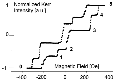
Fig. 2 Polar MOKE hysteresis loop with numbered plateaus.
