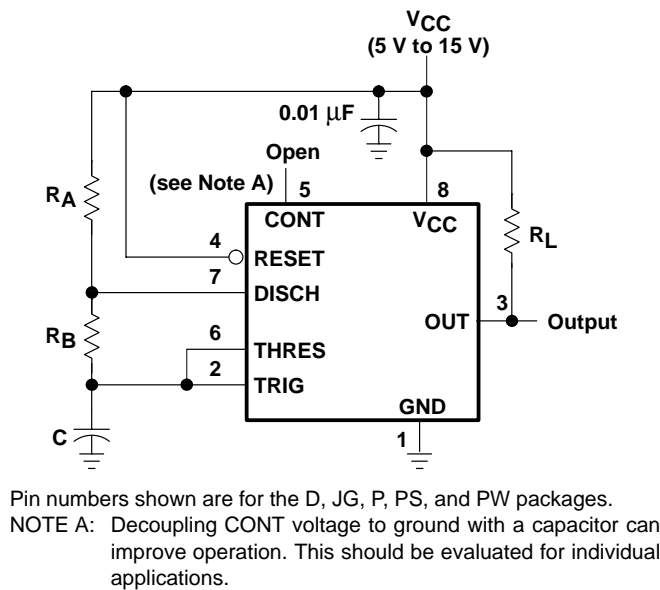
Figure 12. Circuit for Astable Operation
