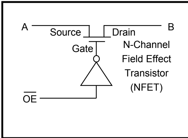
NMOS Switch Circuit Diagram
