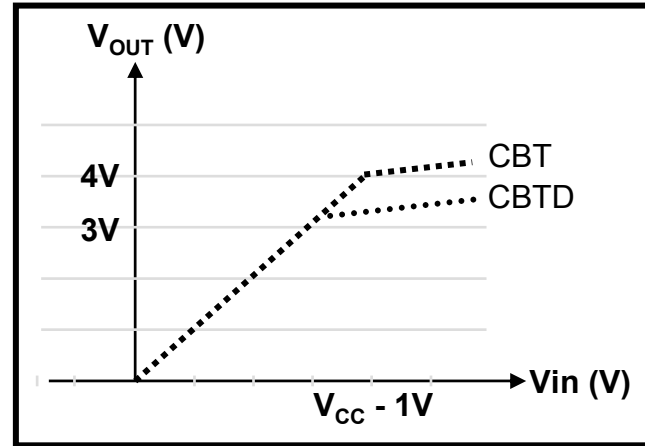
NMOS Switch V_{IN}/V_{OUT} Graph
